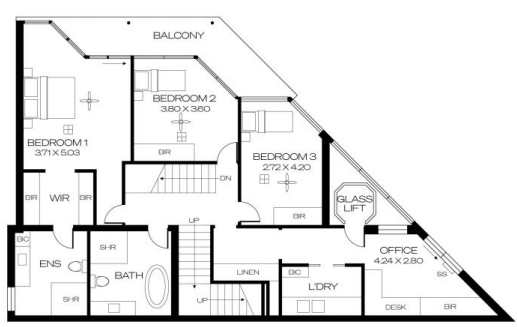
MID LEVEL
