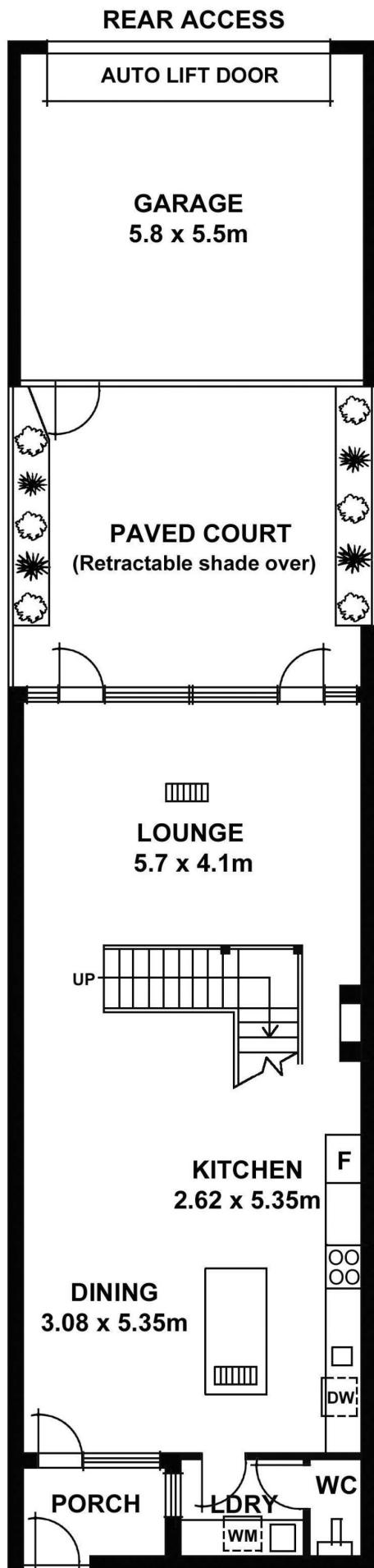
GROUND FLOOR
